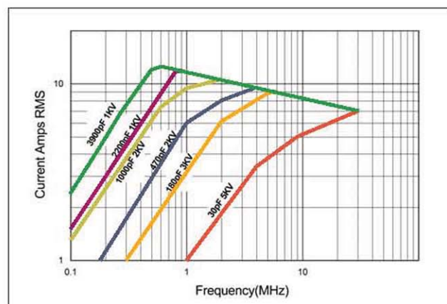
KEC70F Strip Terminals Rated Current vs Frequency
